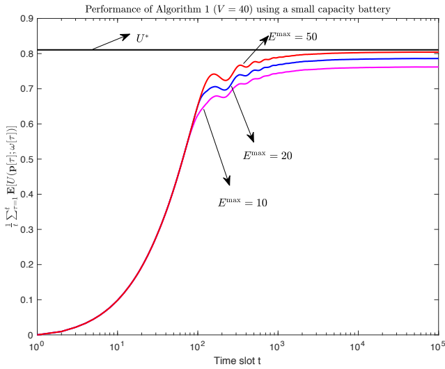
Fig. 6. Utility performance of Algorithm 1 with V = 40 for different E^{\max} in a non-i.i.d. system.
