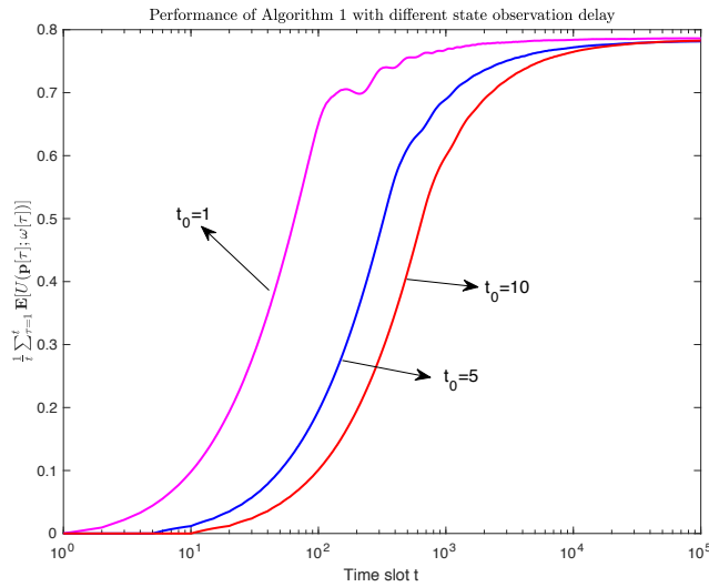
Fig. 7. Utility performance of Algorithm 1 for different system state observation delay in a non-i.i.d. system.
