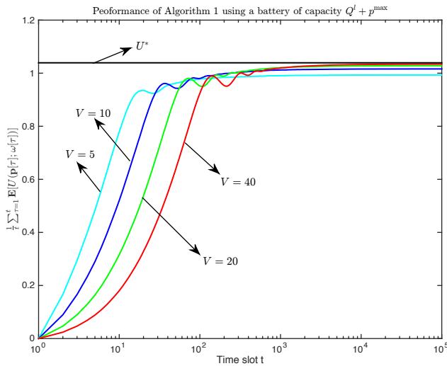
Fig. 1. Utility performance of Algorithm 1 with E[0] = E^{\max} = Q^l + p^{\max} for different V in an i.i.d. system.
