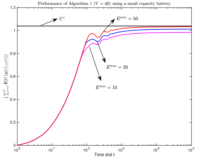
Fig. 2. Utility performance of Algorithm 1 with V = 40 for different E^{\max} in an i.i.d. system.
