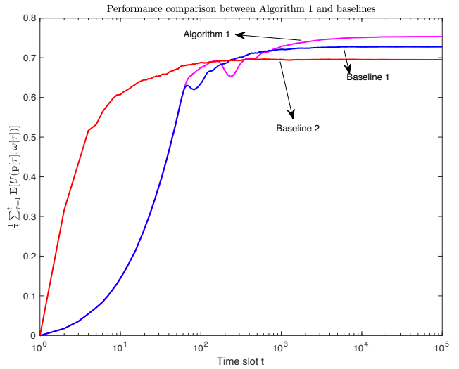
Fig. 4. Performance comparison between Algorithm 1 and two baselines in an i.i.d. system.
