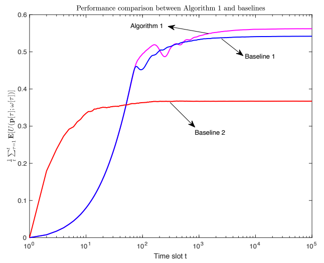
Fig. 8. Performance comparison between Algorithm 1 and two baselines in a non-i.i.d. system.
