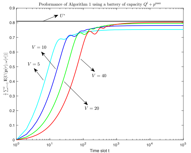
Fig. 5. Utility performance of Algorithm 1 with E[0] = E^{\max} = Q^l + p^{\max} for different V in a non-i.i.d. system.
