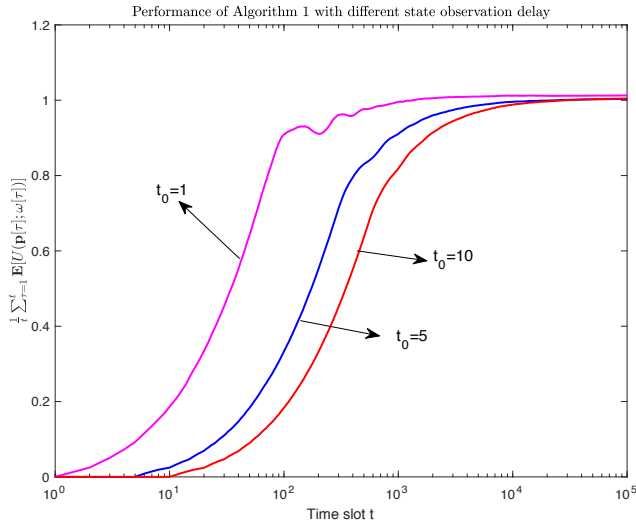
Fig. 3. Utility performance of Algorithm 1 for different system state observation delay in an i.i.d. system.
