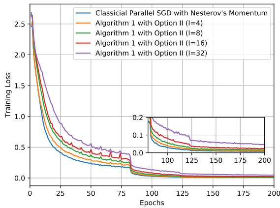
(a) Training loss v.s. epochs
