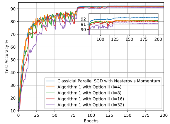
(b) Test accuracy v.s. epochs.
